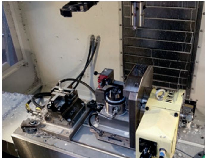
Nikken Rotary Table with device by ZBG.
